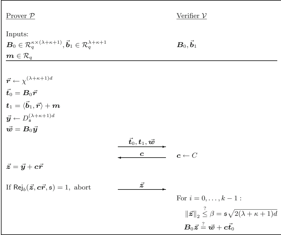
Fig. 4. Opening proof for the commitment scheme. If b = 0 then the protocol is identical to the one described in [ALS20] and uses \text{Rej}_0 defined in Fig. 2. On the other hand, if b = 1 then we apply the new rejection sampling algorithm \text{Rej}_1 in Fig. 2.
