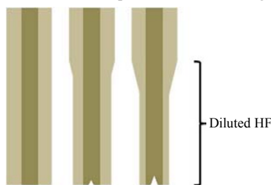
Fig. 2 Fiber tip formation during etching process.
