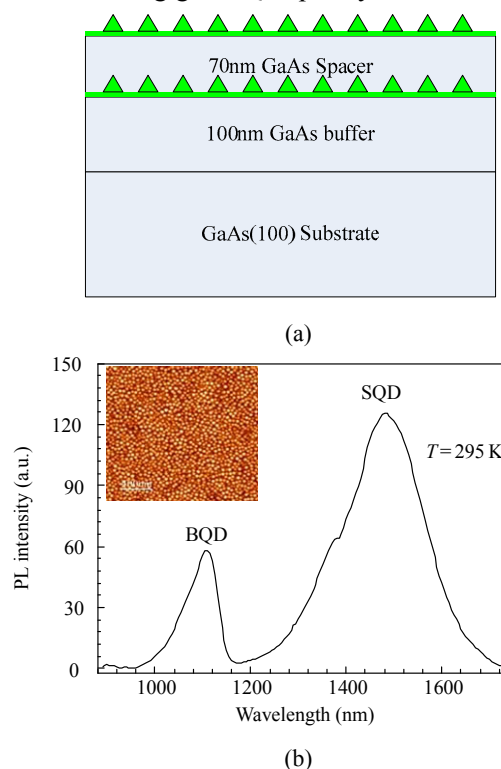
Fig. 1 Schematic of: (a) the hybrid QD structure and (b) PL spectra measured at room temperature ( T=295\text{ K} ) with a laser excitation intensity of 9\text{ W/cm}^2 .
