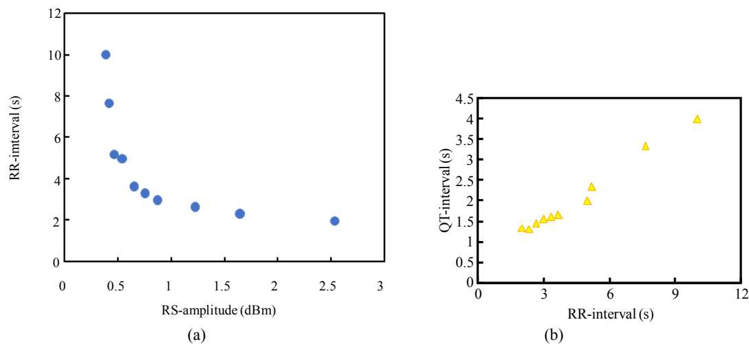
Fig. 5 Further evaluation on the PQQST wave (a) RR intervals against RS amplitudes for the SMS fiber sensor and (b) RR intervals against QT intervals for the SMS fiber sensor.
