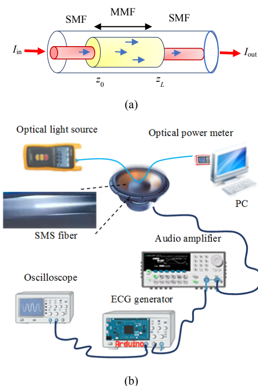
Fig. 2 A schematic set-up for heart rate monitoring (a) an SMS fiber structure and (b) a schematic of the principal operation of heart rate monitoring with the SMS fiber structure attached to the artificial ECG source.
